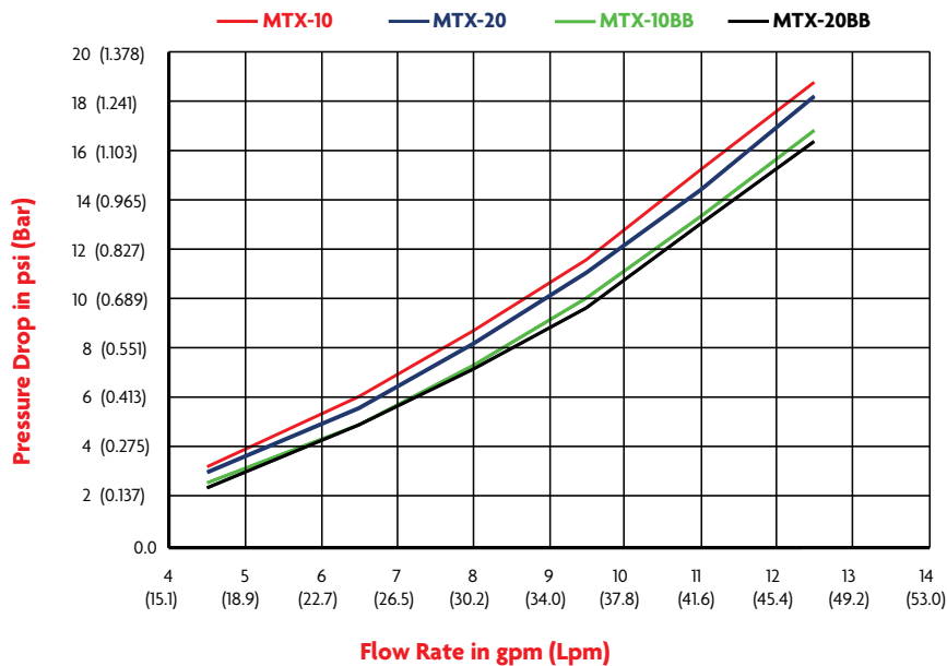
MicroTrex Pressure Drop vs. Flow Rate
